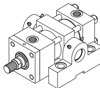
Trunnion mounting block (ISO 8132)
