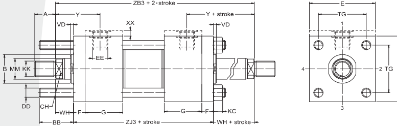
Double rod extended front tie rods
