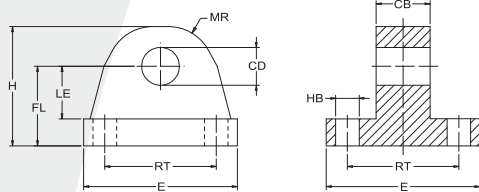
Vertical male counterhinge
