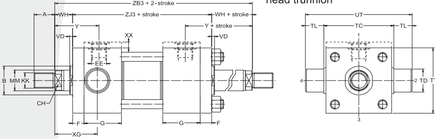
Double rod head trunnion
