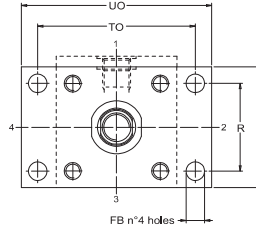
Double rod rectangular front flange
